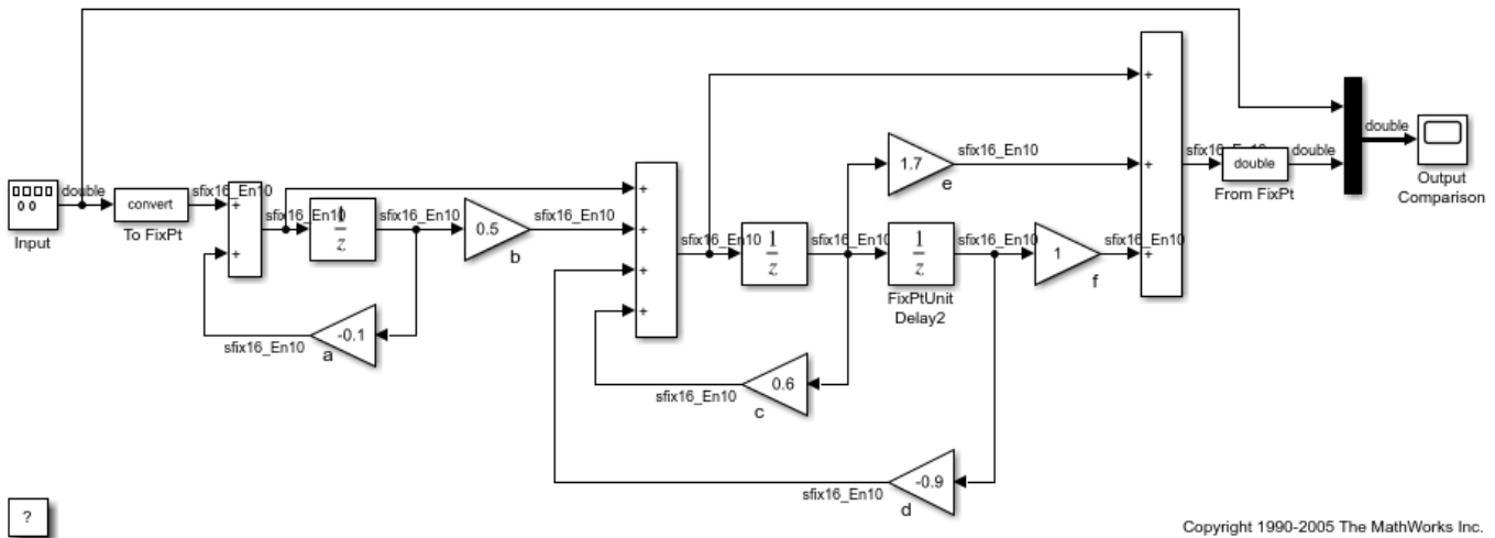
Fixed-Point Series Cascade Form Filter
