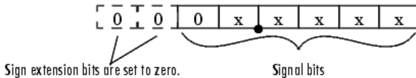
8-bit container for a signed, 6-bit signal that is positive or zero
